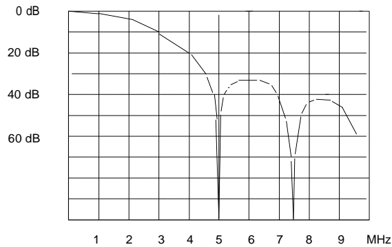
Fig. 3 Spectral density of the 2T Pulse
