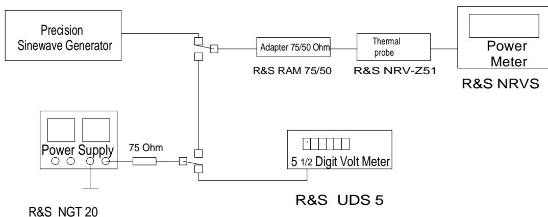
Bild 1 Calibrating the thermal probe and the power meter from DC to 6 MHz
